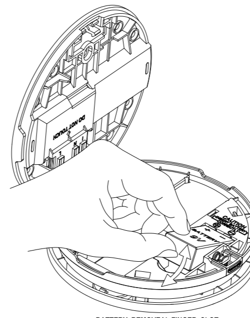
BATTERY REMOVEAL FINGER SLOT
