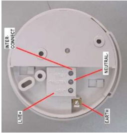
Figure 5 –Wiring & Interconnect facility
