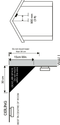
Figure 3i - Positioning the smoke / heat detector Figure 3ii
