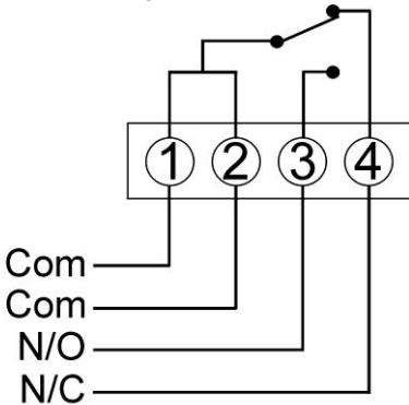
fig 7 – HCP-W(DPS)-SCI additional wiring
