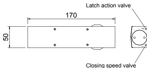
TS1500 BODY
