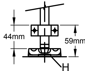
B1 - 3405 BOTTOM BOLT KEEP ALTERNATIVE BOTTOM KEEP AS SUPPLIED WITH STEEL DOOR VERSION (285SD)
