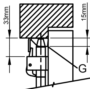
C1 - 3405A TOP TRIP KEEP ALTERNATIVE SURFACE MOUNTED TOP TRIP KEEP AS SUPPLIED WITH STEEL DOOR VERSION (285SD)
