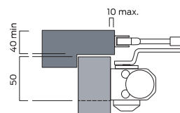
Fig.1 Door mount - pull side UK CA CE
