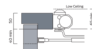
Fig.61 Transom mount - push side UK CA CE
