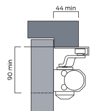
Fig.66 Parallel arm - push side UK CA CE
