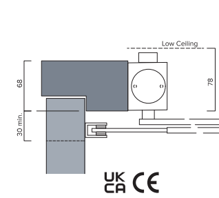
Fig.61 Transom mount push side
