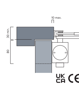
Fig.1 Door mount pull side
