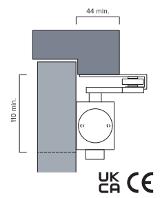
Fig.66 Parallel arm push side mount
