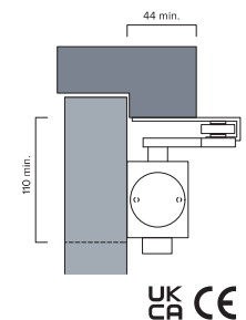
Fig.66 Parallel arm push side mount
