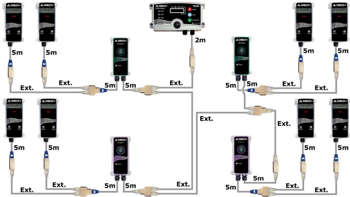
1 x Central Display; 2 x CO 2 Sensors; 2 x O 2 Sensors; 8 x Alarms
