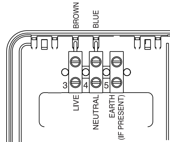
Figure 6 - Recessed Wiring
