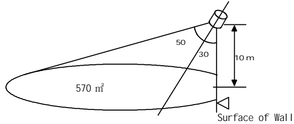
Wall Mounting(Surface type) In case of 30° Inclination
