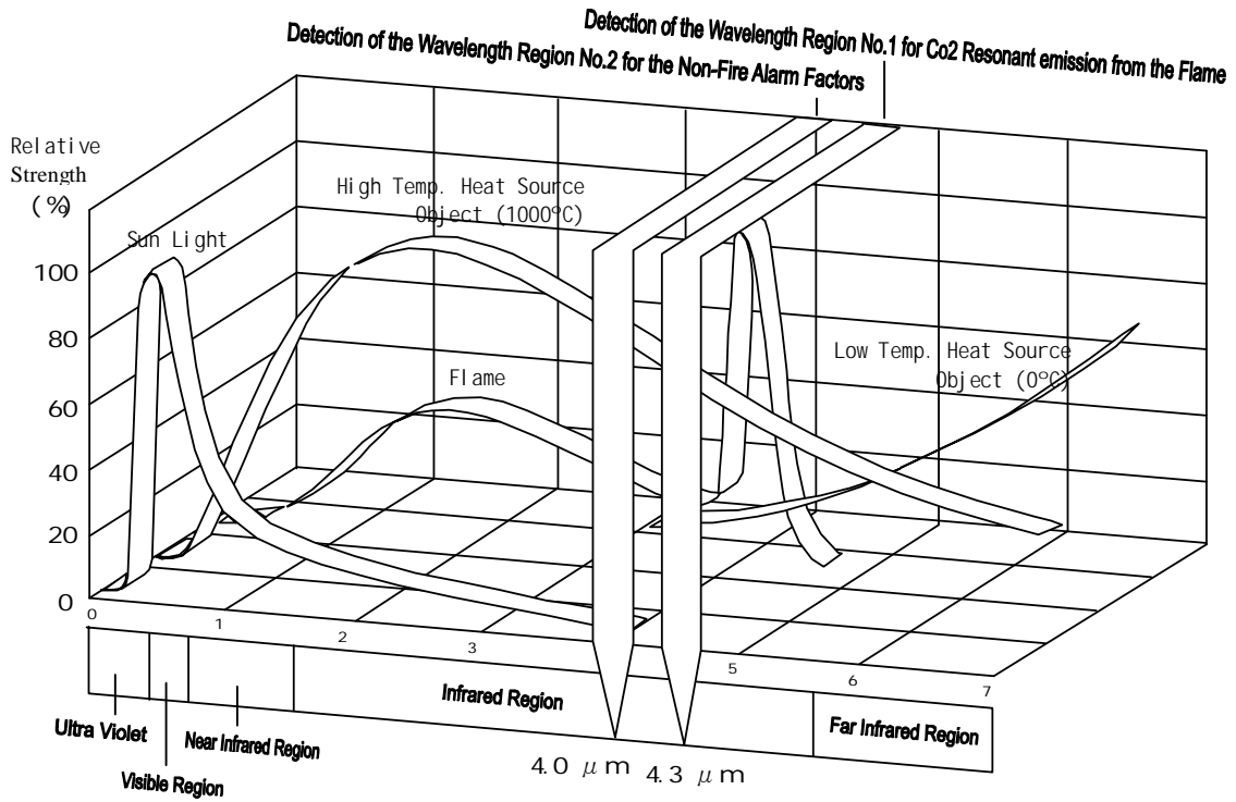
Fig-1 : Various Light Spectrum Emission Strength
