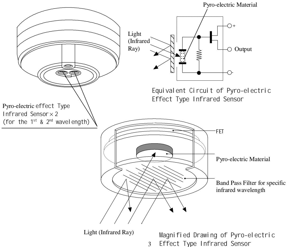
Fig-1 : Structure & Equivalent Circuit Infrared Spot Type Flame Detector
