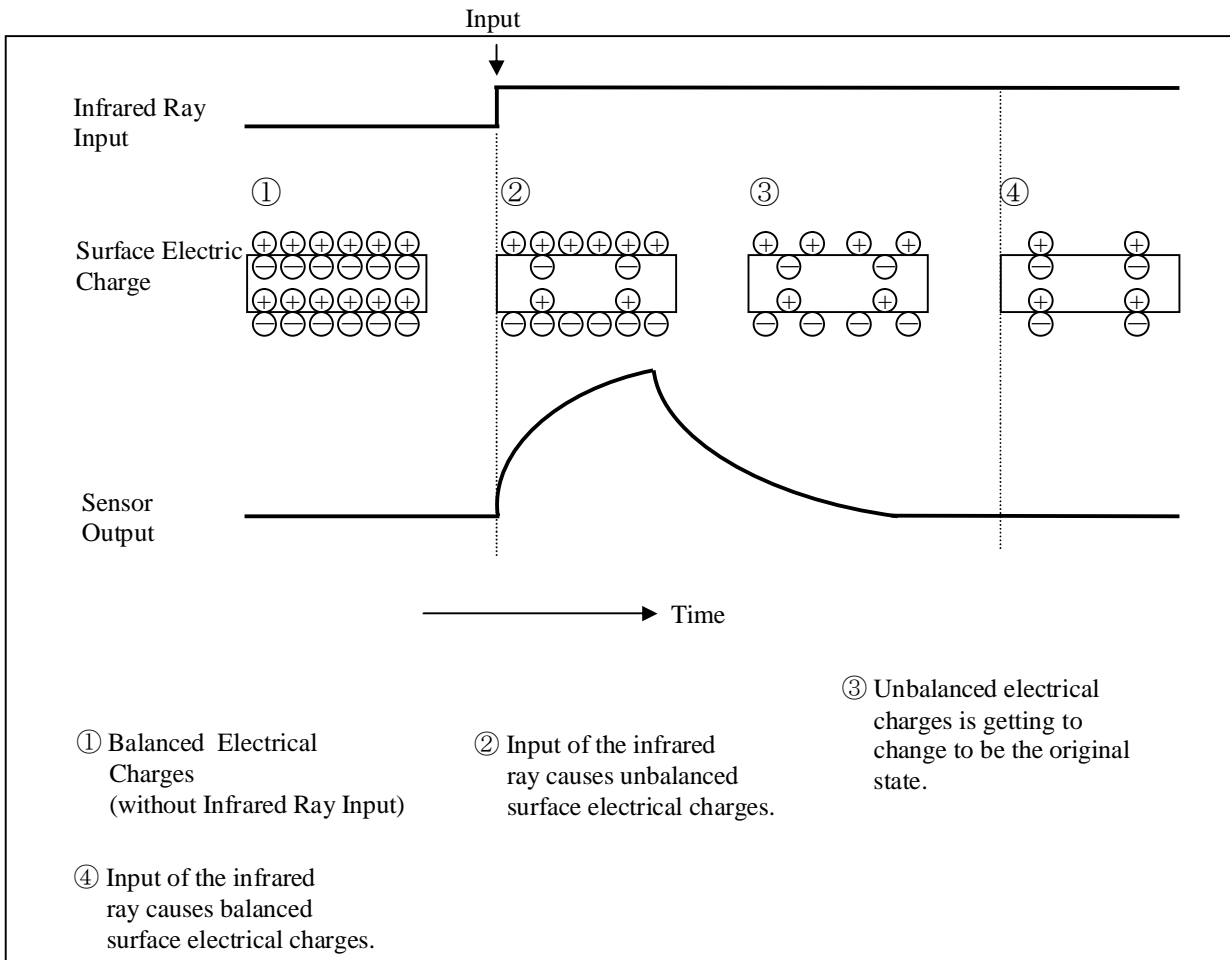
Fig-2 : Concept Drawing of Pyro-electric Effect
